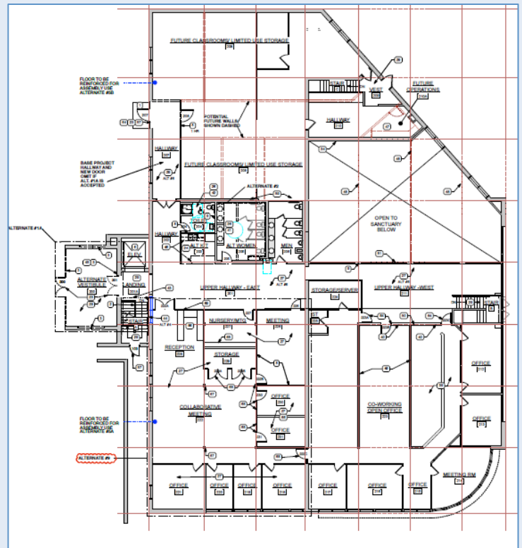
UPPER LEVEL
